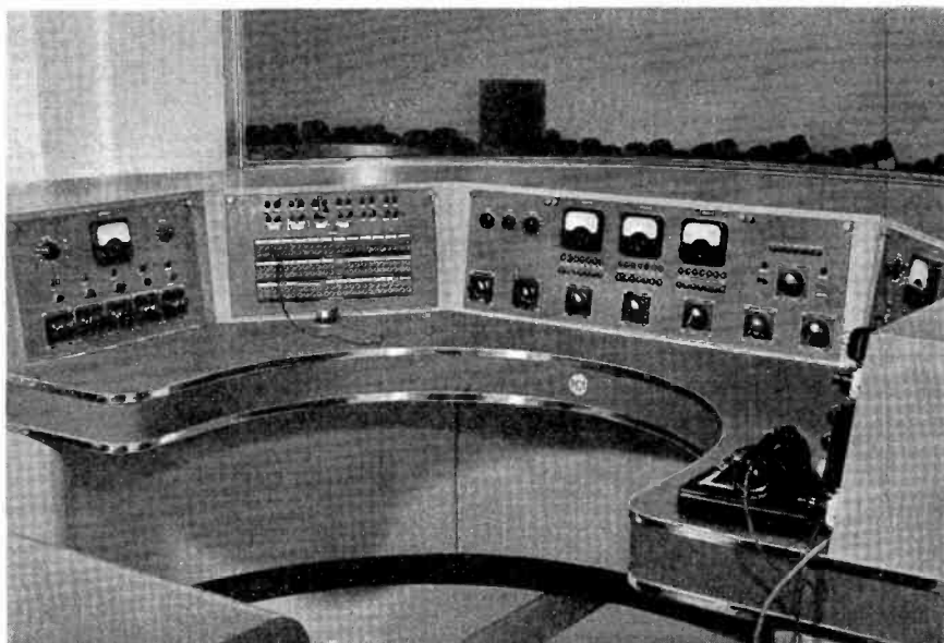
One of the studios used interchangeably by FM station WBRL and AM station WJBO. RCA-Type 44-BX Microphones are used in this studio, in the smaller announce-type studio, and in the large, auditorium-type studio.
